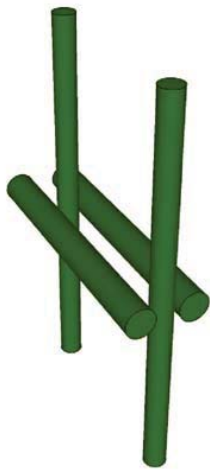
Twin Wire Detail Double Horizontal Wires Ø 8mm & Single Vertical wires Ø 6mm
