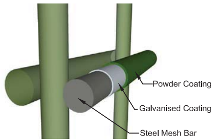
Single Welded Bar Breakdown
